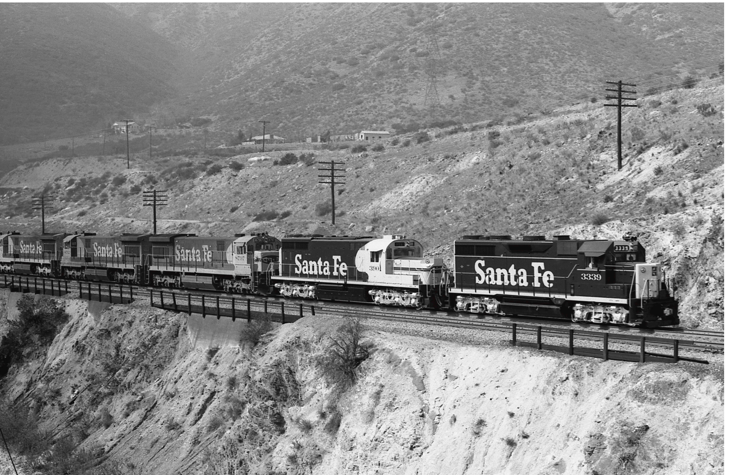
Former RSD15 number 9826, now CRSD20 3901 dead-in-tow on Cajon eastbound at Blue Cut, 1977.
